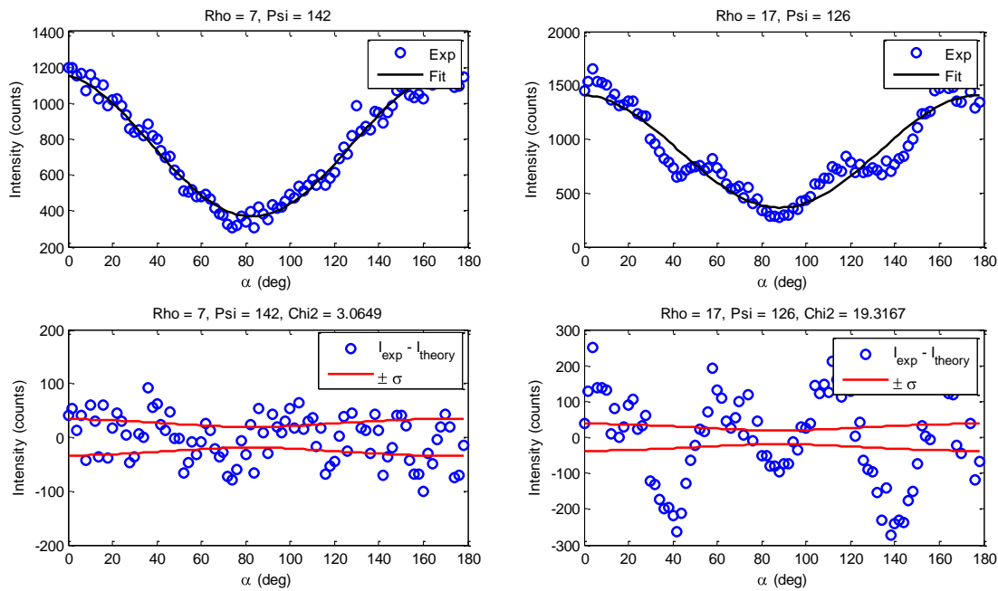
Figure S4. Illustration of the data filtering procedure. Raw data are plotted with blue circles. The fitting theoretical curve is displayed in black. Below: corresponding plot of the residuals I_{\text{exp}} - I_{\text{theory}} . The range \pm the standard deviations is represented by red curves. Left: in this case, \chi^2 = 3.1 is below the rejection threshold. The retrieved values are \psi = 142^\circ \pm 1^\circ , \rho = 7^\circ \pm 1^\circ . Right: in this case, the measurement is affected by intensity fluctuations. The fit leads to \chi^2 = 9 , which is above the rejection threshold. This dataset is discarded. Note that both cases (left and right) pass the “number of photon” test, since their total intensity is above the 5000 photons threshold. The difference between the two data is in their fit quality ( \chi^2 value), introduced to remove the data containing artifacts that would lead to a biased psi (fluctuations of the membrane, motion of the sample, defocusing, bleaching...).
