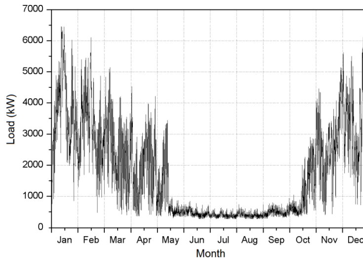
Fig.4. Heating network load (kW)
