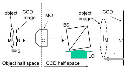
Fig. 1 – Holographic microscopy setup. CCD: CCD sensor; BS: beam splitter; LO: Reference wave (Local Oscillator); MO: Microscope Objective; O: MO optical center; F and F': object and image focal points of MO. M: object position; M': image of the object position.
