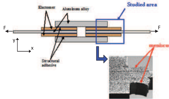
Fig. 2. Four-lap-joint samples
