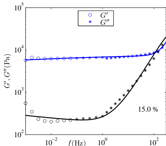
Fig. 7: Rheology of the 15% acrylamide gel. Rheometrical (open circles) and AFM (stars, with standard deviations shown) experimental data. Solid lines are the best model fits.
