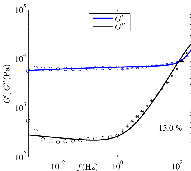
Fig. 6: Rheology of the 15% acrylamide gel. Rheometrical (open circles) and AFM (stars) experimental data. Solid lines are the model best-fitting curves.
