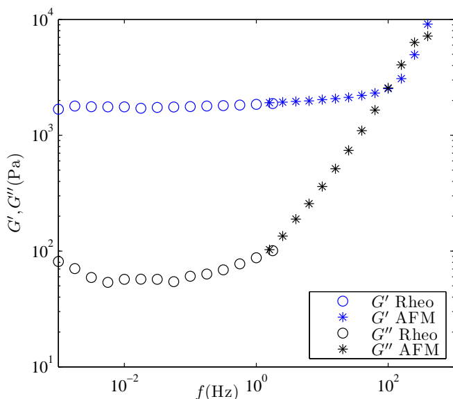
Fig. 1: Superposition of rheometrical (open circles) and AFM measurements (stars). The acrylamide content is 10% in this case. Typical error bars are around 10%. T = 25^\circ\text{C} .
