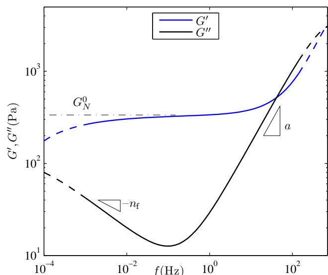
Fig. 2: Significance of the model parameters: G_N^0 (plateau modulus), n_f (slope of G'' at low frequencies), and a = b (slopes of G' and G'' at high frequencies). \omega \sim 1/\lambda_{\max} corresponds to the intersection of G' and G'' occurring for very low frequencies (not shown). G_1 corresponds to a higher plateau modulus in G' for \omega \sim 1/\lambda_1 , but is well above our data.
