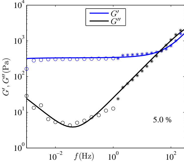
Fig. 3: Rheology of the 5% acrylamide gel. Rheometrical (open circles) and AFM (stars) experimental data. Solid lines are the model best-fitting curves.
