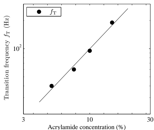
Fig. 8: Evolution of transition frequency f_T vs. concentration. The power law exponent is 1.6 \pm 0.1 .
