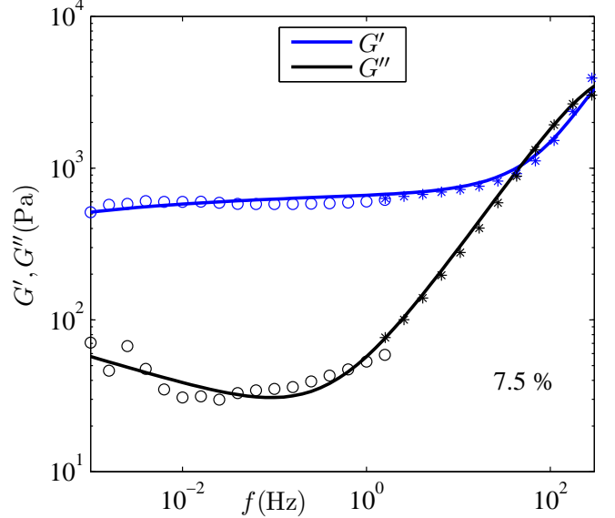
Fig. 4: Rheology of the 7.5% acrylamide gel. Rheometrical (open circles) and AFM (stars) experimental data. Solid lines are the model best-fitting curves.
