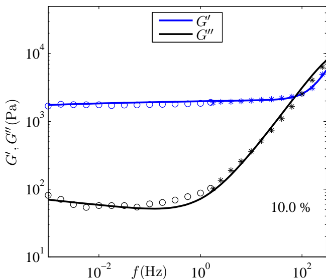
Fig. 5: Rheology of the 10% acrylamide gel. Rheometrical (open circles) and AFM (stars) experimental data. Solid lines are the model best-fitting curves.
