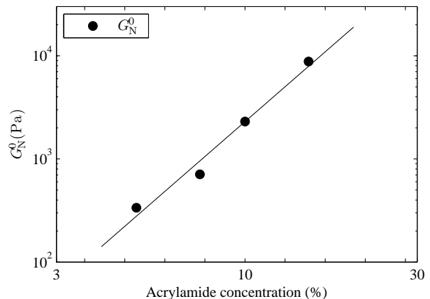
Fig. 7: Evolution of gel modulus G_N^0 vs. concentration. The slope of the power law exponent corresponds to 3.0 \pm 0.3 .
