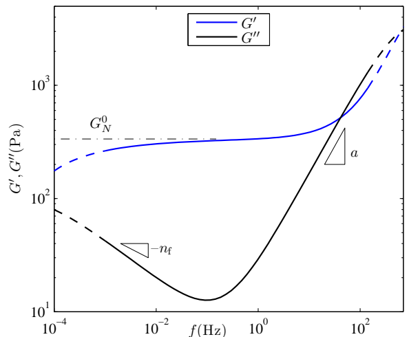
FIG. 2: Significance of the model parameters G_N^0 , n_f , and b = a . \lambda_{\max} is not shown but should appear at lower frequencies at the intersection of G' and G'' occurring for \omega \sim 1/\lambda_{\max} . This does not occur in such gels since the flow region is not reached at low frequencies. Similarly G_1 corresponds to a higher plateau modulus in G' but is well above our data, this being also the case for \lambda_1 .
