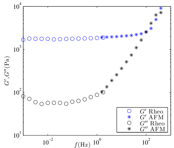
FIG. 1: Superposition of rheometrical and AFM microrheological measurements. The acrylamide content is 10% in this case. Typical error bars (not shown) are around 10%. T = 25^\circ\text{C} .
