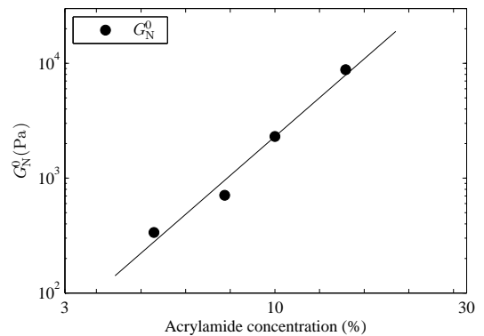
FIG. 4: Evolution of gel moduli G_N^0 vs. concentration. The slope of the power law exponent corresponds to 3.0 \pm 0.3 .
