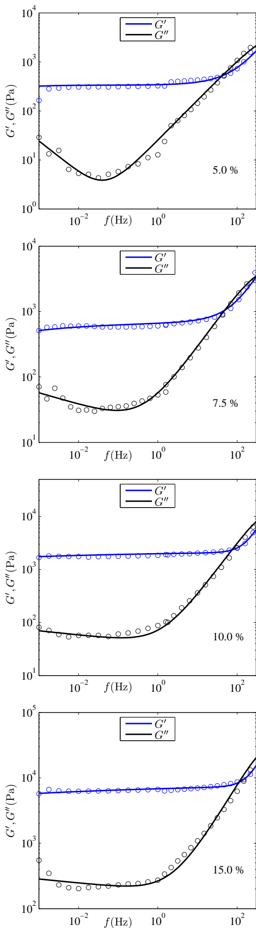
FIG. 3: Gel rheology: 5%, 7.5%, 10% and 15% acrylamide concentrations. Open circles are experimental data whereas solid lines are the model best-fit curves.
