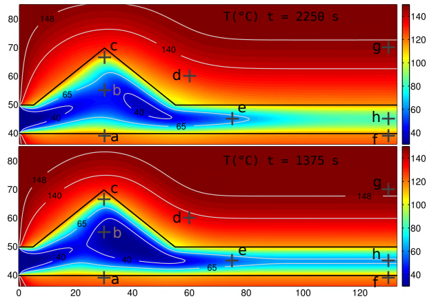
Figure 8. (Color online) Temperature as a function of time, for the geometry characterized by (d, L) = (20 \text{ mm}, 50 \text{ mm}) , at t = 1375 \text{ s} and t = 2250 \text{ s} , with isotherm lines (40, 65, 140, 148)°C. The letters a-h indicates the locations where the temperature evolution is observed in Fig. 6.
