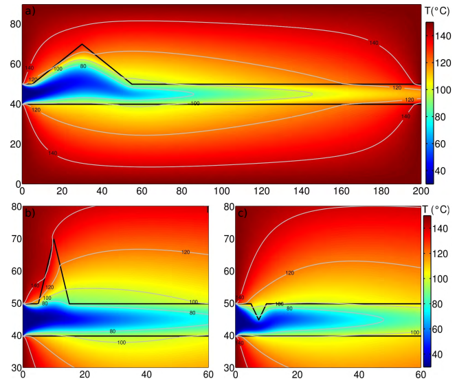
Figure 2. Temperature maps at steady state for various asperity shapes: (a) (d, L) = (20 \text{ mm}, 50 \text{ mm}) , (b) (d, L) = (20 \text{ mm}, 10 \text{ mm}) , (c) (d, L) = (-5 \text{ mm}, 5 \text{ mm}) . The black lines delimit the fracture embedded in the rock. The gray lines are isotherm lines (80, 100, 120 and 140°C).
