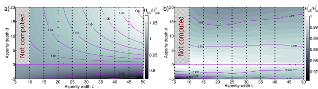
Figure 10. (Color online) Color maps as a function of the asperity depth d and width L of (a) the hydraulic aperture computed with the lubrication approximation, H_{hb}^* = H_{hb}/H_{hb}^{||} , and (b) the ratio between the hydraulic aperture computed with LBM, H_{LB}^* , and the one computed with the lubrication approximation, H_{hb}^* . The dots indicate the computed values from which the map is deduced. The purple lines are isolines.
