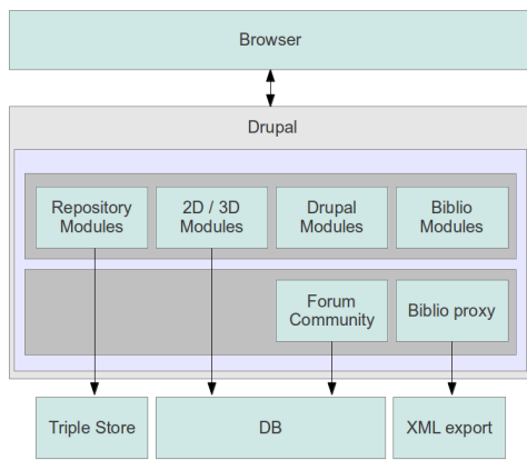
Figure 2: System architecture of the AKGDC Framework.
