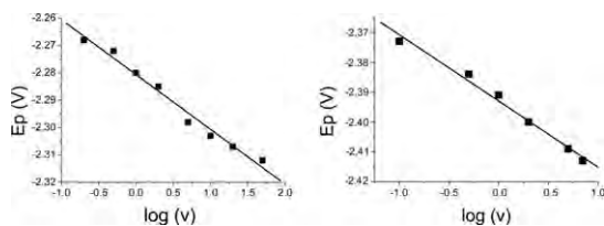
Fig. 2 Cyclic voltammetry of \approx 5 \times 10^{-3} mol L -1 acetophenone at a glassy carbon electrode. Variation of the peak potential in V vs. Fc/Fc + with the logarithm of the scan rate in [PMIm][NTf 2 ] (left) and in [BMMIm][NTf 2 ] (right).
