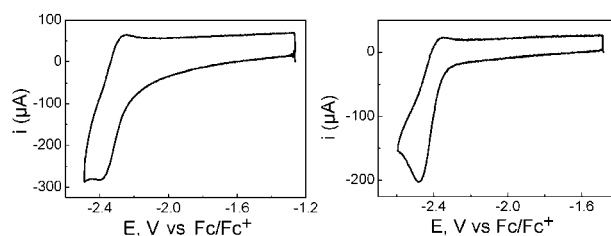
Fig. 3 Cyclic voltammetry of \approx 5 \times 10^{-3} mol L -1 acetophenone showing reversibility. Left, in [EMIm][NTf 2 ] at 200 V s -1 . Right, in [EMMIm][NTf 2 ] at 30 V s -1 .
