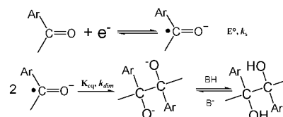
Scheme 1 Radical–radical dimerization mechanism involved in the electrodimersation of acetophenone
