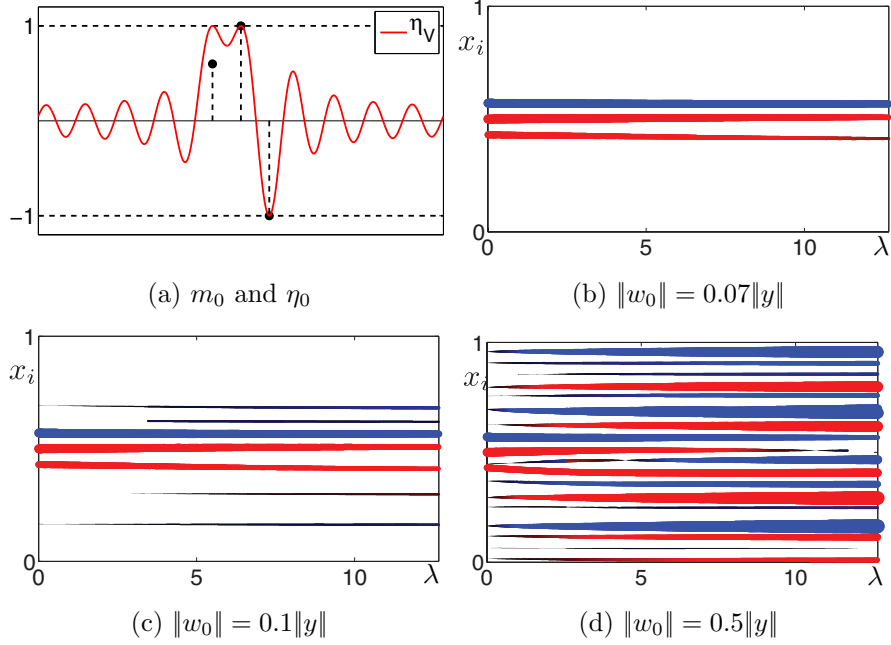
Figure 2: Same plots as Figure 1 except that the solutions of \mathcal{P}(\Phi m_0 + \lambda w_0) are displayed instead of those of \mathcal{P}_\lambda(\Phi m_0 + w) . possibly a condition on its norm). The following pre-certificate appears naturally in our analysis.
