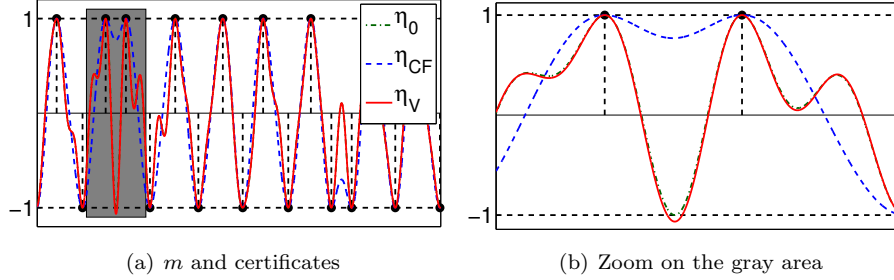
Figure 4: Example of measure for which \eta_V \neq \eta_0 . known as the Lasso [31] in statistics. Indeed, defining the linear operator \Psi through
