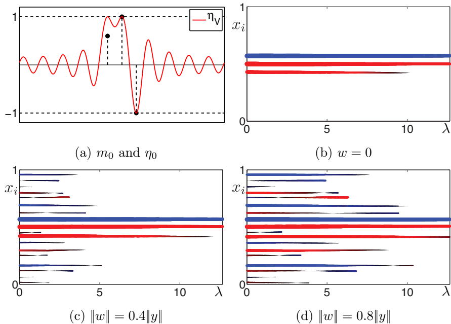
Figure 1: (a) Input measure m_0 , and corresponding minimal norm certificate. (b,c,d) Regularization paths \lambda \mapsto \tilde{m}_\lambda that are solutions of \mathcal{P}(\Phi m_0 + w) for three different noise levels \|w\| . Each “strip” represents the evolution of a spike as \lambda varies. The color refers to the sign of the spike (blue for negative and red for positive) and the (vertical) width is proportional to its amplitude. The exact location is given by the middle of each band.
