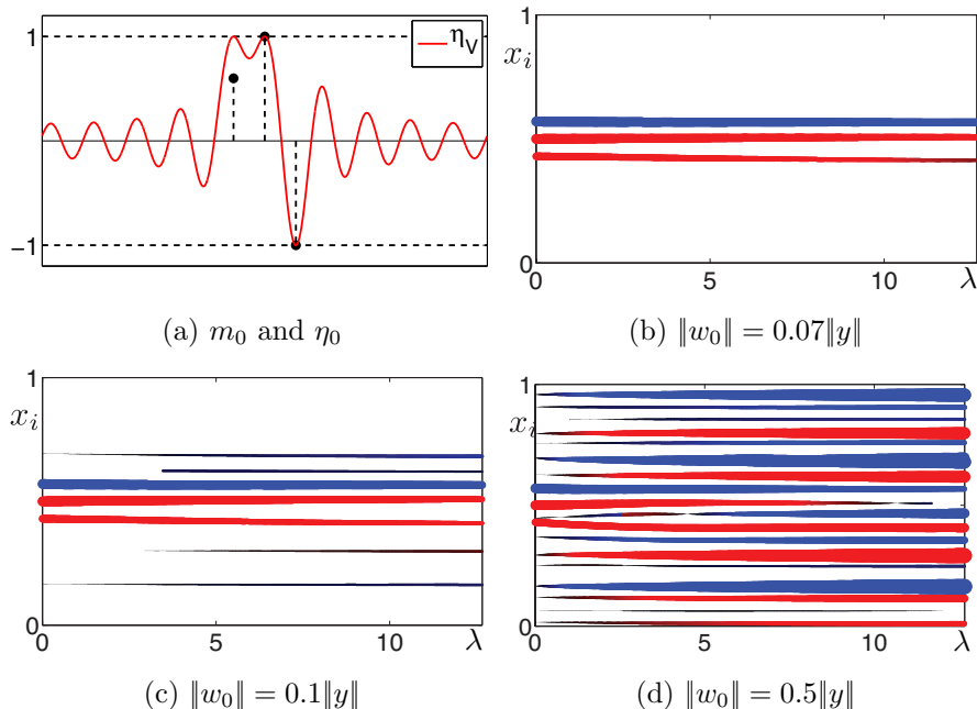
Figure 2: Same plots as Figure 1 excepted that the solutions of \mathcal{P}(\Phi m_0 + \lambda w_0) are displayed instead of those of \mathcal{P}(\Phi m_0 + w) .
