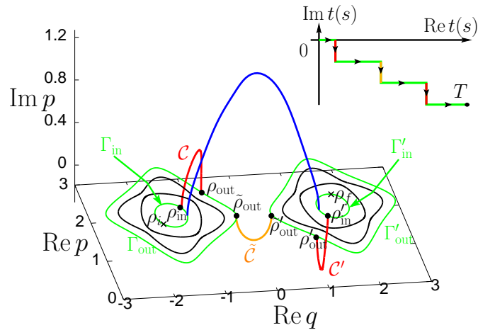
Figure 3: (Color online) Phase space of the Hamiltonian (8) (thin black lines) for a_1 = 1 , a_2 = -0.55 , |b| = 0.05 , and \phi = \pi/4 , plotted together with two different complex trajectories at energy E \simeq 0.035 that connect an arbitrarily chosen initial point \rho_i \equiv (p_i, q_i) on the real torus \Gamma_{\text{in}} with an arbitrarily chosen final point \rho_f \equiv (p_f, q_f) on the symmetric counterpart \Gamma'_{\text{in}} [both tori are plotted in (light) green]. The (red and orange) arcs are half of the complex orbits (ii) \mathcal{C} , \mathcal{C}' , and (iv) \tilde{\mathcal{C}} described in the text. Together with the connecting pieces of \Gamma_{\text{out}} and \Gamma'_{\text{out}} , they constitute a complex trajectory that results from the time path depicted in the upper right inset. The (dark) blue line is a complex orbit lying on a part of the complex manifold that directly connects the symmetric tori \Gamma_{\text{in}} and \Gamma'_{\text{in}} (see Fig. 4). These two trajectories are plotted in a reduced three-dimensional complex phase space spanned by (\text{Re} p, \text{Re} q, \text{Im} p) .
