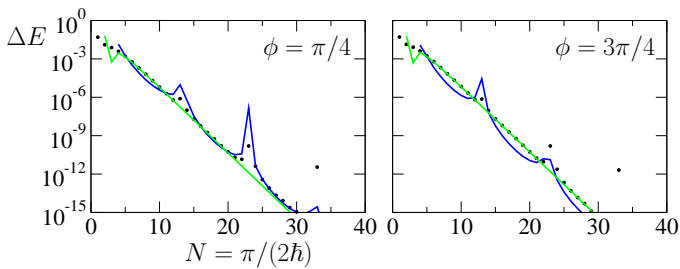
Figure 7: (Color online) Quantum and semiclassical level splittings \Delta E_0 associated with the eigenstates that are most strongly localized on the centers of the four symmetric islands, for the Hamiltonian (8a) with the parameters a_1 = 1 , a_2 = -0.55 and |b| = 0.001 , plotted versus N \equiv \pi/(2\hbar) for \phi = \pi/4 (left panel) and \phi = 3\pi/4 (right panel). The (black) dots represent the exact results, the dark (blue) solid lines correspond to the resonance-assisted semiclassical splittings obtained with the semiclassical formula (21), and the light (green) straight lines show the direct splittings given by Eq. (26). The effect of the resonance is significantly reduced as compared to Fig. 5, and the splittings no longer display systematic variations as a function of the rotation angle \phi .
