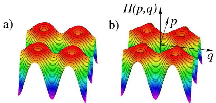
Figure 1: (Color online) Graph of (p, q) \mapsto H(p, q) on the fundamental domain [-\pi, \pi] \times [-\pi, \pi] where H is given by Eq. (8) with a_1 = 1 , a_2 = -0.55 , \phi = 0 and (a) b = 0 ; (b) |b| = 0.05 .
