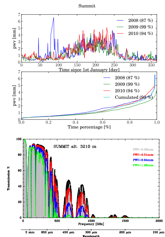
Fig. A.6. PWV statistics ( top ) and transmission curves ( bottom ) for Summit (Greenland). The transmission curve for the first decile of PWV is in grey, and the quartiles of PWV are given by red: 25%, blue: 50%, green: 75%.
