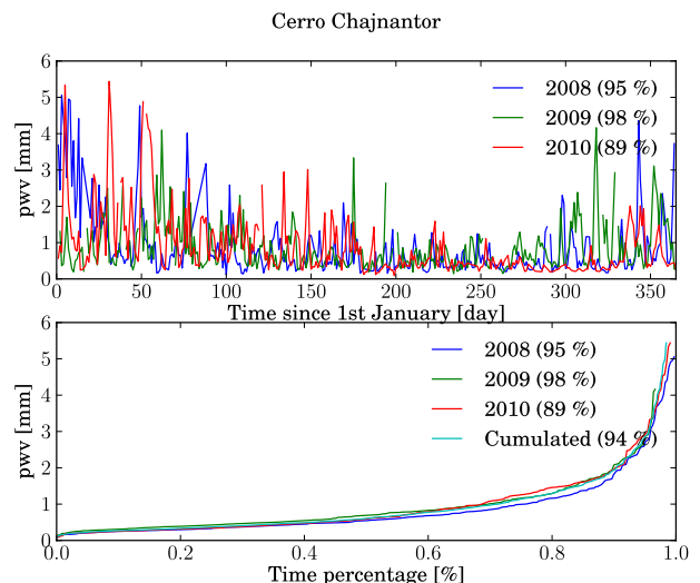
Fig. 3. Same as Fig. 2 for Cerro Chajnantor in Chile. The satellite profiles were truncated at the altitude of the mountain summit. Note the different scale range of PWV compared to Fig. 2.
