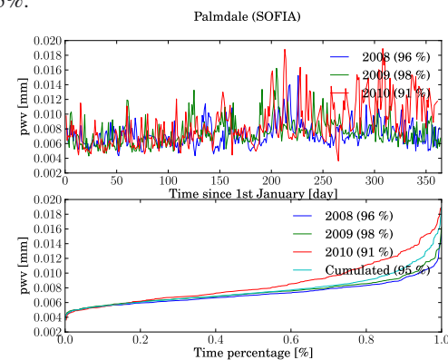
Fig. A.8. PWV statistics for Palmdale USA, at a stratospheric altitude of 12 km.
