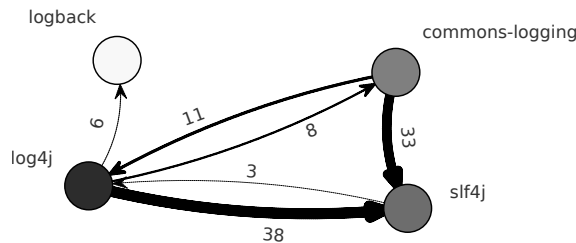
Figure 8: Migration graph of the logging category
