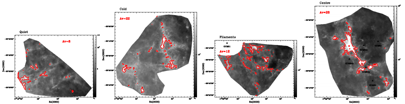
Fig. 7. Individual column-density maps of the sub-regions expressed in visual extinction A_V (in the range of A_V -values for the PDF with the contour level of the lower limit used for fitting the slope in the high-density tail of the PDF (Fig. 5). The corresponding values are given in each panel.
