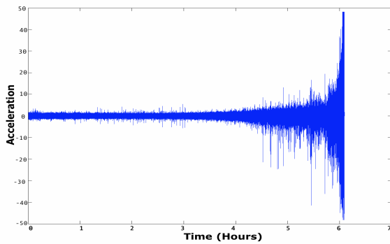
Fig. 2. Example of raw signal extracted from bearing testbed
