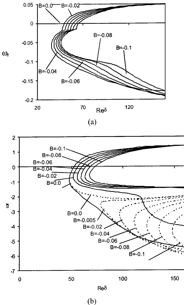
FIG. 5. Comparison of the neutral curves \omega_r = f(Re_\delta) in the stationary disk boundary layer obtained at different B : (a) convectively unstable areas, (b) absolutely unstable areas (dashed lines indicate second family).
