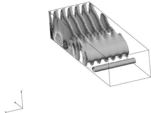
FIG. 16. Iso-surface of the fluctuations of the axial velocity component at Re_R=13\ 200 , \eta=0 , t=60 , showing large spiral arms expanding from the vertical boundary layer to the geostrophic core and related to a centrifugal instability.
