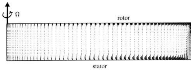
FIG. 8. Base flow. Velocity field in the meridional plane (r, z, 0) at Re_R = 3000 . Batchelor-type flow composed of two boundary layers on the rotating and stationary disks separated by a solid body rotating core.
