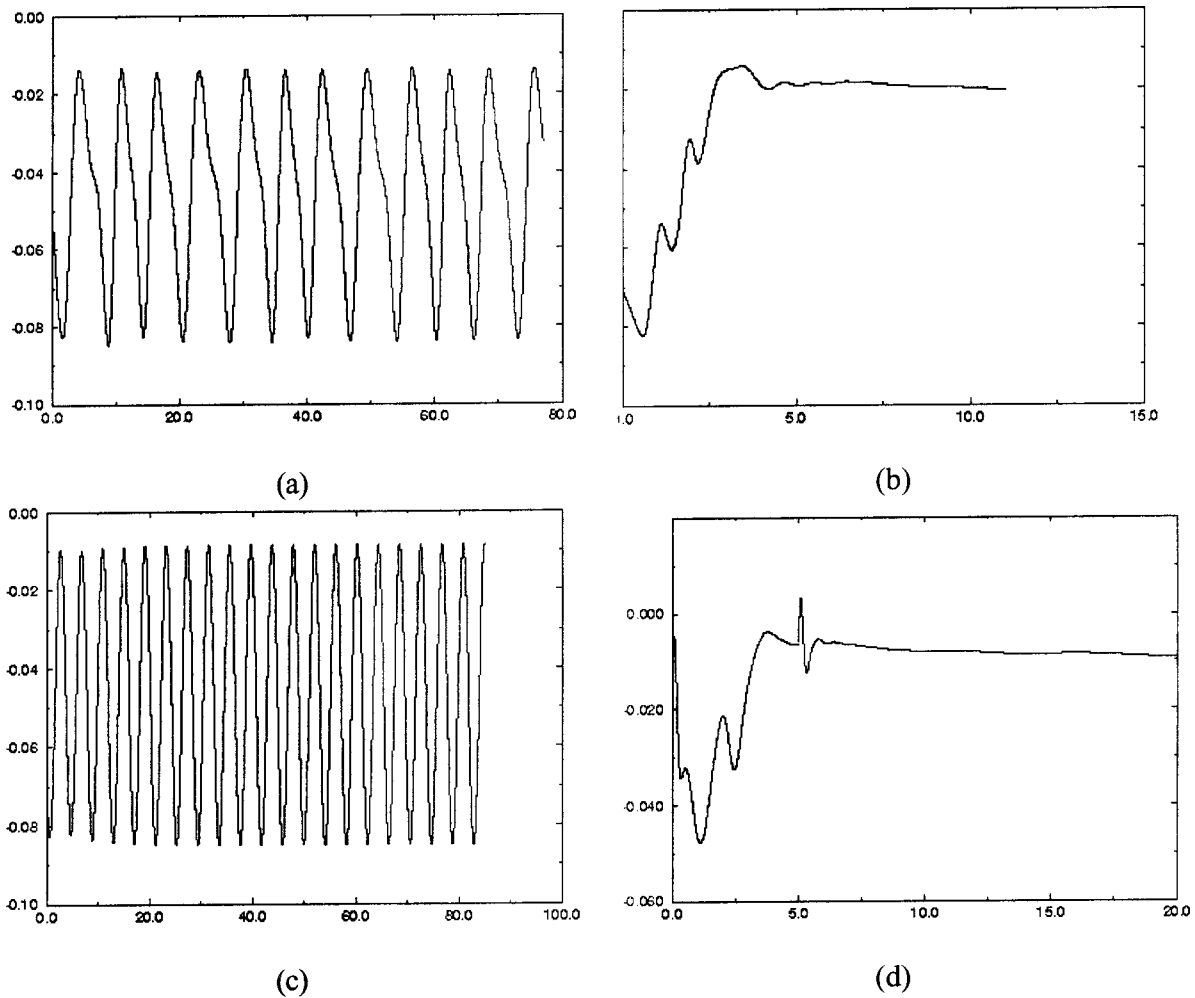
FIG. 13. (a) and (b) Time histories of the axial component of the velocity obtained at Re_R=13\,200 , \eta=0.0 : (a) outer cylinder attached to the stator, (b) outer cylinder attached to the rotor and using (a) as initial condition. (c) and (d) Time histories obtained at Re_R=13\,200 , \eta=3.5 : (c) outer cylinder attached to the stator; (d) linear azimuthal velocity profile as boundary condition and using (c) as initial condition.
