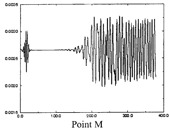
FIG. 9. Time histories of the axial component of the velocity in the stationary disk boundary layer at Re_R = 13\,200 , \eta = 0 and at different monitoring points A, B, M.
