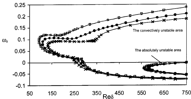
FIG. 6. Comparison of the neutral curves \omega_r = f(Re_\delta) of the absolutely and convectively unstable flow obtained for B = 0.1 (crosses), 0.04 (dots), and 0.0 (squares). The rotating disk boundary layer.
