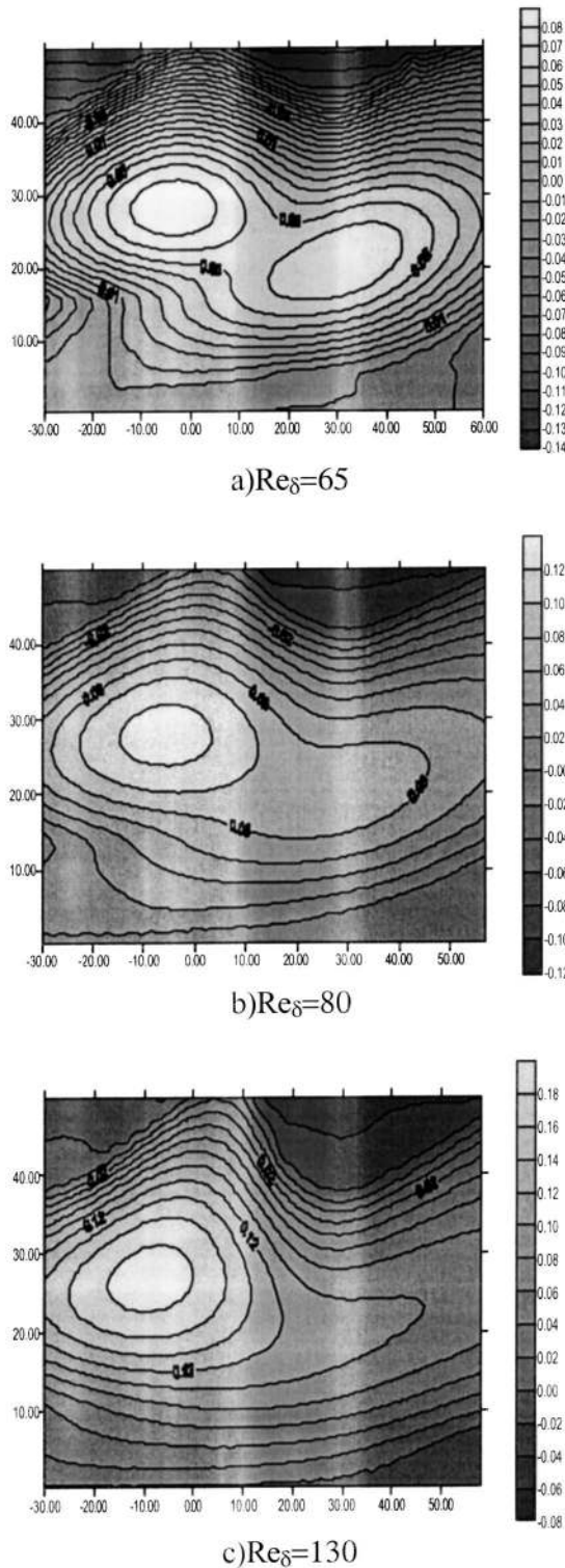
FIG. 3. Iso-lines of \omega_1 = \text{const} in the stationary disk boundary layer and at different local Reynolds numbers.
