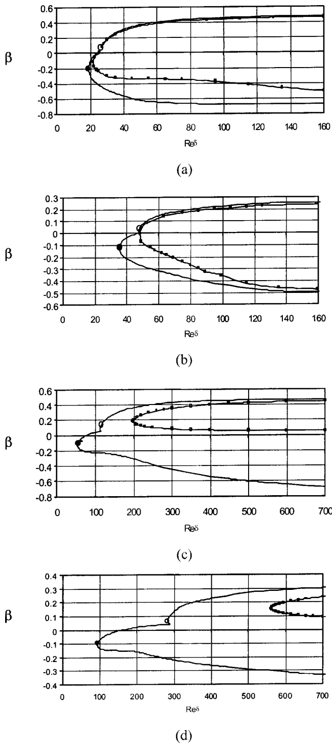
FIG. 7. Comparison of the neutral curves \beta=f(\text{Re}_{\delta}) of the absolutely (black squares) and convectively (solid line) unstable flow obtained for [(a) and (b)] the Bödewadt flow and the stationary disk boundary layer, respectively; [(c) and (d)] the Ekman flow and the rotating disk boundary layer, respectively. The critical points of type I and type II are marked by the white and black dots, respectively.
