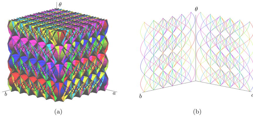
Fig. 2 (a) Tipping surfaces in the 3D parameter space (a, b, \theta) , and (b) their cross-sections, namely tipping curves, in the 2D planes (a, \theta) and (b, \theta) .
