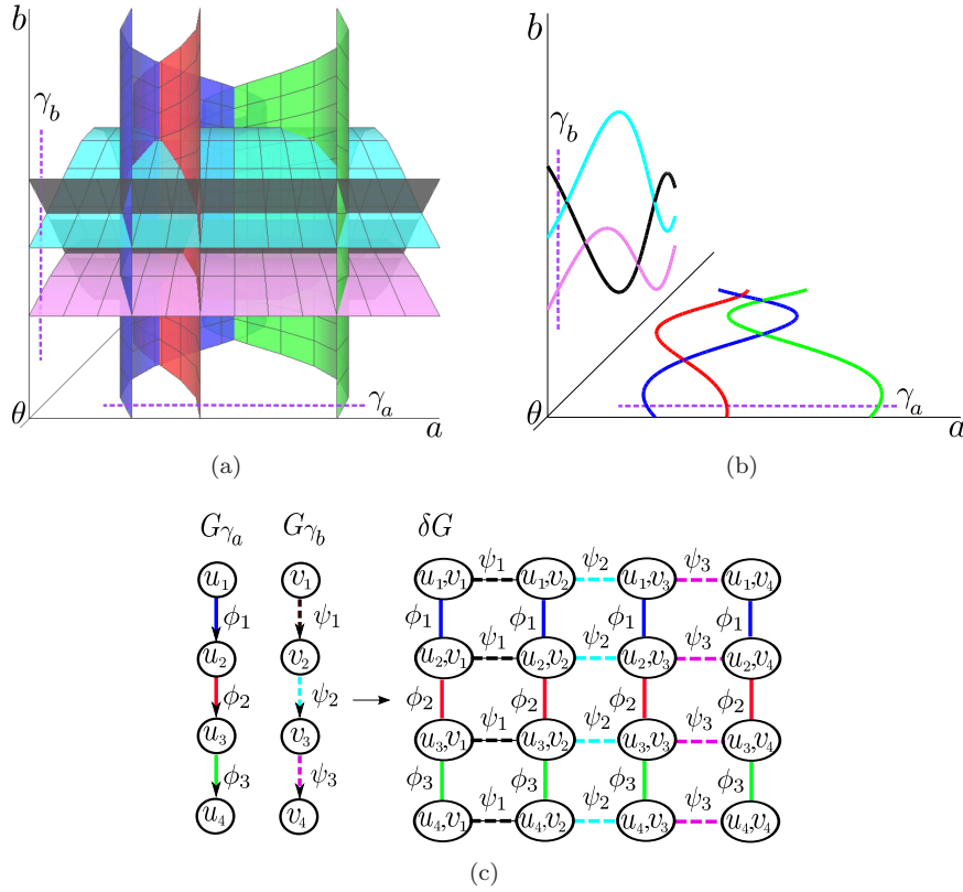
Fig. 9 Generation of a partial graph \delta G from two graphs G_{\gamma_a} and G_{\gamma_b} associated to cuts \gamma_a and \gamma_b respectively.
