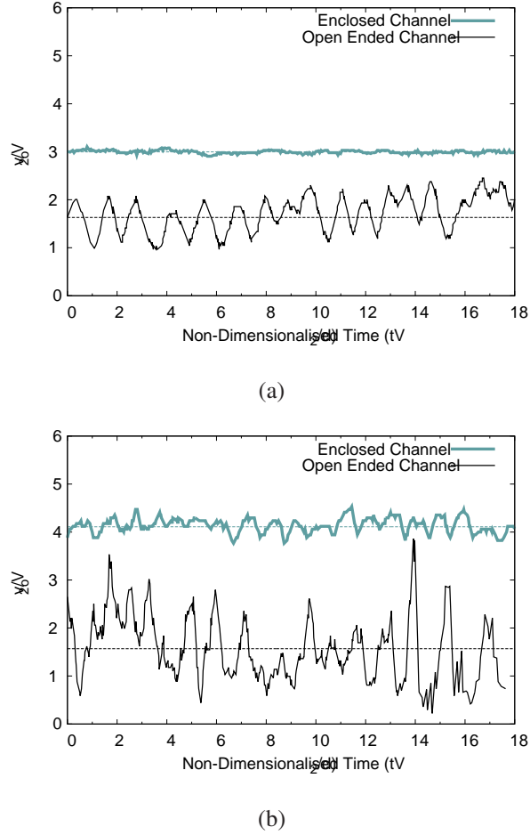
FIG. 5. Velocity, non-dimensionalised by the reference velocity V_0 , versus dimensionless time for both the enclosed and open-ended channels. (a) For a channel of width 0.38 cm and (b) for a channel of width 0.12 cm. Large fluctuations are observed for open-ended channels. The mean value V_2 for each case is indicated with a dashed line. The velocity in the enclosed-channel data is offset by +2 to improve clarity.
