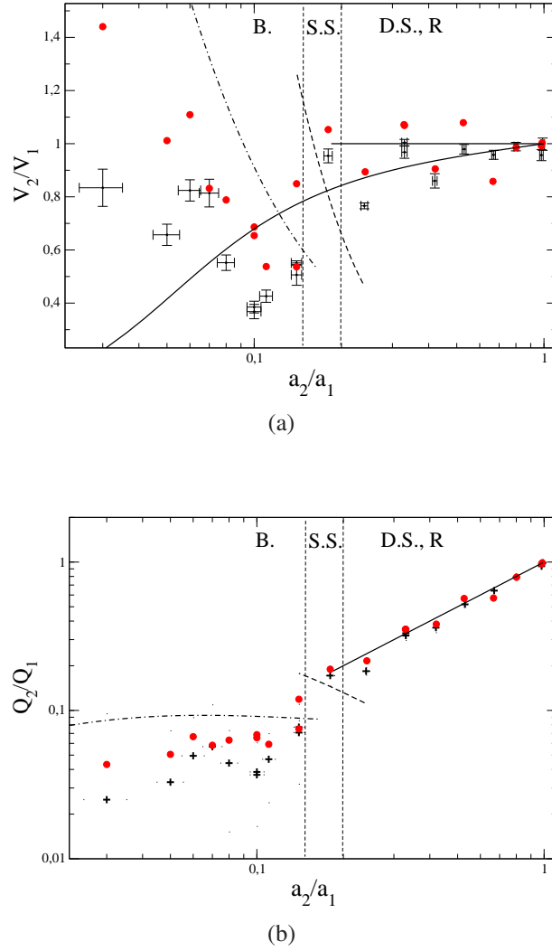
FIG. 11. (a) Comparison of the experimental data of Fig. 4 with theoretical predictions. Analytical prediction: horizontal solid line - random foam structure (R) in the narrow channel; dashed line - staircase structure (S.S.), eq. (17); dotted-dashed line - bamboo structure (B. S.), eq. (16) ( A = 0.19 \text{ cm}^2 , h = 0.1 \text{ cm} and a_2 = 4x/(1+x) in cm, with x = a_2/a_1 ). The functions are plotted in the domains of existence of the corresponding structure, as observed experimentally. The vertical dashed lines that separate these domains are not strict frontiers, and some fluctuations are observed. In the “random domain”, adjacent to the staircase domain, one data point corresponds to a double staircase structure (D.S.), for which a special treatment would lead to a better theoretical prediction. The prediction of eq. (14), determined from the experimental values of the foam structure and the velocity in the wide channel, is given as \bullet . The curved solid line is the velocity ratio expected for a Newtonian fluid 37 . The analytical expression is given in Annex. (b) Same data for the fluxes (without the result for a Newtonian fluid).
