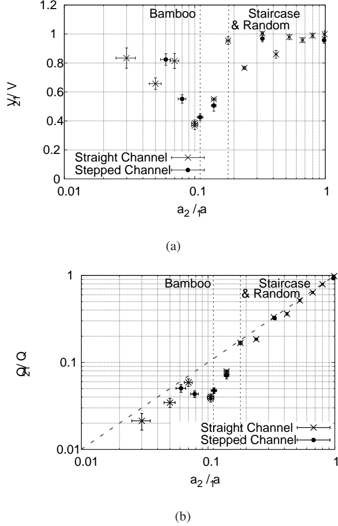
FIG. 4. Dependence of (a) the velocity ratio, V_2/V_1 , and (b) the flux ratio, Q_2/Q_1 , on the channel width ratio, a_2/a_1 , for the enclosed channels. The bubble size is R = 0.25 cm and a_1 + a_2 = 4 cm. The dotted vertical lines indicate the limits of the transition zone in which a mixture of single staircase and bamboo foam was observed in the narrow channel. The regions of the graph in which only bamboo or where only staircase or random foams were observed are labeled.
