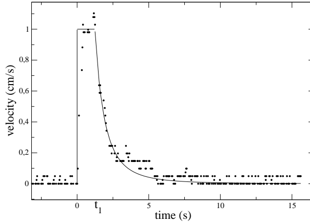
FIG. 13. Velocity of a bamboo film in a narrow channel as a function of time. ● Experimental data. Solid line, for t > t_1 : prediction of eq. (25) v(t) = v_0 [1 + (t - t_1)/\tau]^{-3} , with the adjustable parameter \tau = 2s . v_0 is the maximal velocity, reached by the lamella between t = 0 , the time at which a pinned bubble burst, and t_1 = 1.24s , the time at which a new film was pinned at the channel outlet.
