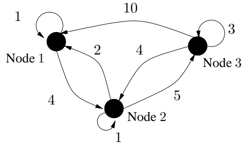
Figure 1: Activity network
