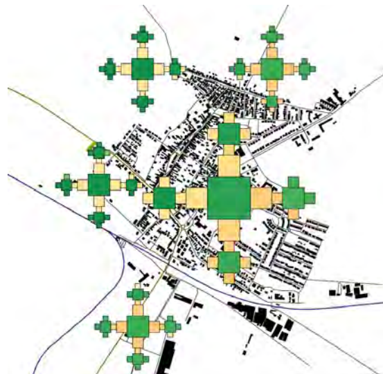
Example of evaluation for a theoretical multifractal.
