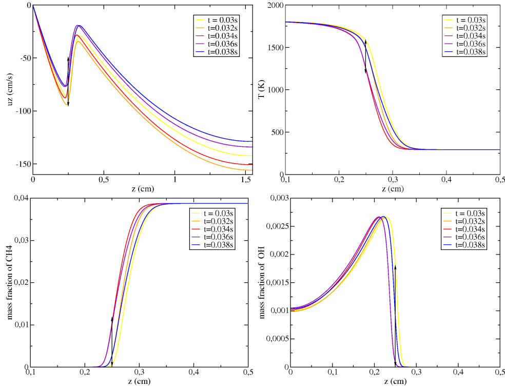
FIG. B.2. Top: time variations of axial velocity u_z (left) and temperature T (right) profiles. Bottom: mass fraction profiles for Y_{\text{CH}_4} (left) and Y_{\text{OH}} (right). Position z = 0.25\text{ cm} is indicated.
