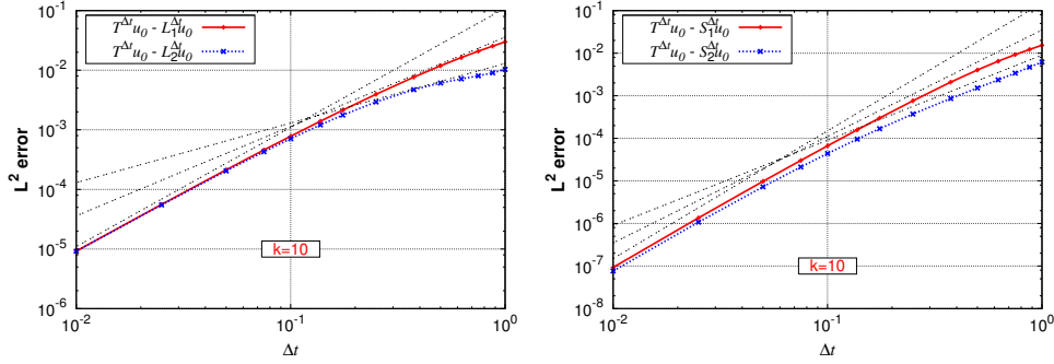
FIG. 3.2. 1D KPP with k = 10 . Local L^2 errors for several splitting time steps \Delta t for Lie (left) and Strang (right) splitting schemes. Dashed lines with slopes 2, 1.5, and 1 (left), and with 3, 2.5, and 2 (right) are depicted.
