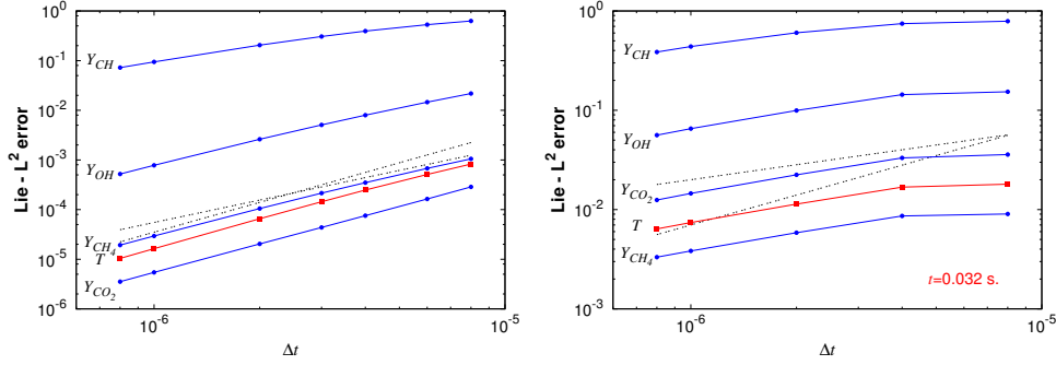
FIG. 4.3. Local (left) and global (right) L^2 errors for the Lie scheme for temperature T and species Y_{CH_4} , Y_{CO_2} , Y_{OH} , and Y_{CH} . Lines with slope of 2 and 1.5 (left), and of 1 and 0.5 (right) are depicted.
