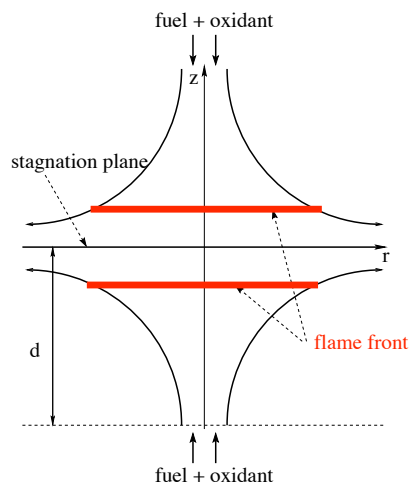
FIG. B.1. Schematic configuration of the counterflow, premixed flames.
