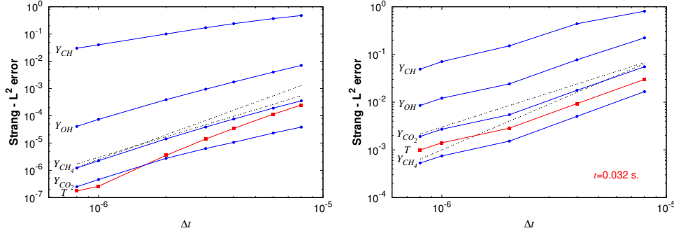
FIG. 4.4. Local (left) and global (right) L^2 errors for the Strang scheme for temperature T and species Y_{CH_4} , Y_{CO_2} , Y_{OH} , and Y_{CH} . Lines with slope of 3 and 2.5 (left), and of 2 and 1.5 (right) are depicted.
