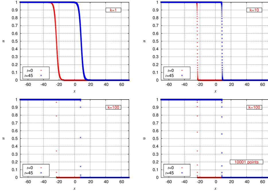
FIG. 3.1. 1D KPP. Numerical quasi-exact solutions at t = 0 and t = 45 for k = 1 (top left), 10 (top right) and 100 (bottom left) with a discretization of 5001 points. Bottom right: case k = 100 with 10001 points of discretization.
