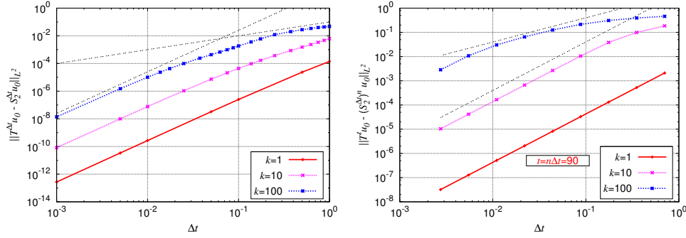
FIG. 3.4. 1D KPP. \mathcal{S}_2 -Strang local (left) and global (right) L^2 errors for several splitting time steps \Delta t and k = 1, 10, \text{ and } 100 . Dashed lines with slopes 3 and 1 (left), and with 2 and 1 (right) are depicted.
