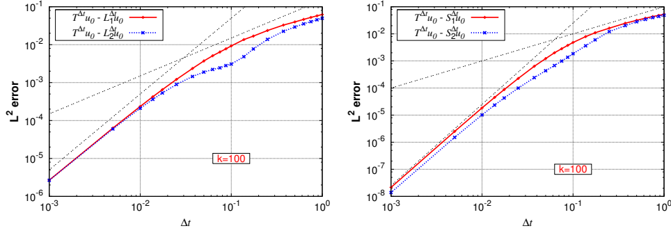
FIG. 3.3. 1D KPP with k = 100 . Local L^2 errors for several splitting time steps \Delta t for Lie (left) and Strang (right) splitting schemes. Dashed lines with slopes 2 and 1 (left), and with 3 and 1 (right) are depicted.
