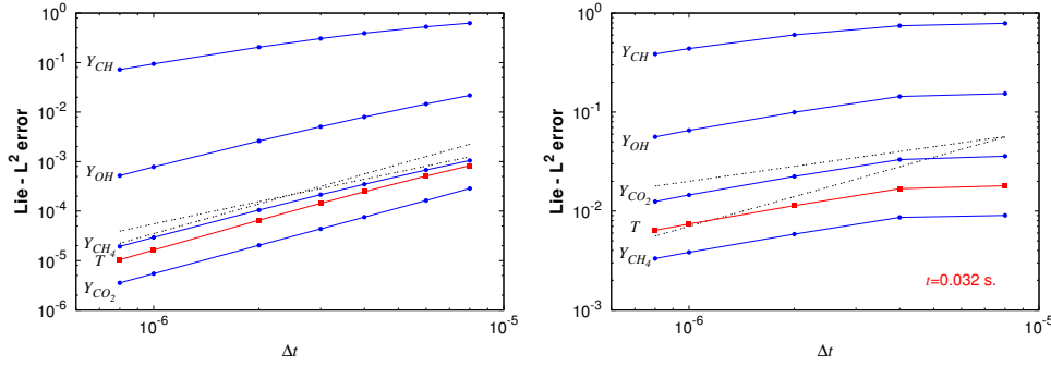
FIG. 4.3. Local (left) and global (right) L^2 errors for the Lie scheme for temperature T and species Y_{\text{CH}_4} , Y_{\text{CO}_2} , Y_{\text{OH}} , and Y_{\text{CH}} . Lines with slope of 2 and 1.5 (left), and of 1 and 0.5 (right) are depicted.
