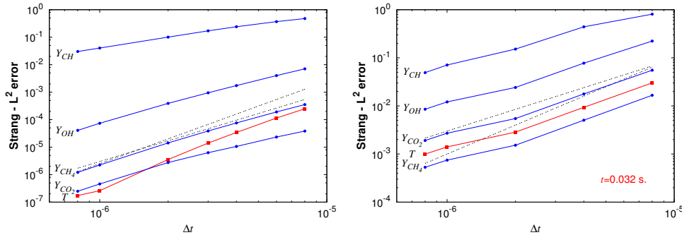
FIG. 4.4. Local (left) and global (right) L^2 errors for the Strang scheme for temperature T and species Y_{\text{CH}_4} , Y_{\text{CO}_2} , Y_{\text{OH}} , and Y_{\text{CH}} . Lines with slope of 3 and 2.5 (left), and of 2 and 1.5 (right) are depicted.
