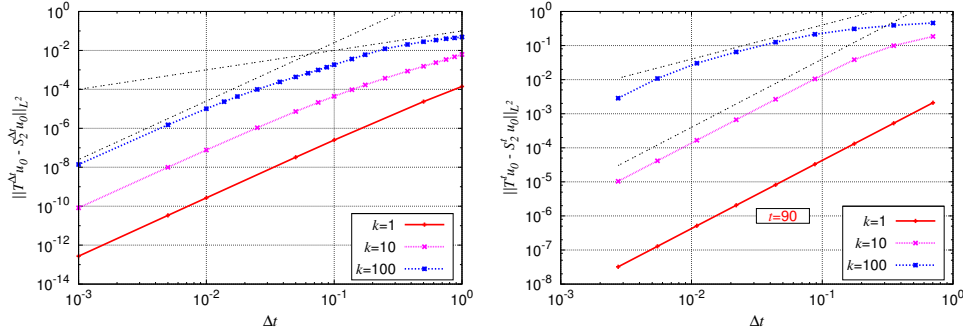
FIG. 3.4. 1D KPP. S_2 -Strang local (left) and global (right) L^2 errors for several splitting time steps \Delta t and k = 1, 10, \text{ and } 100 . Dashed lines with slopes 3 and 1 (left), and with 2 and 1 (right) are depicted.
