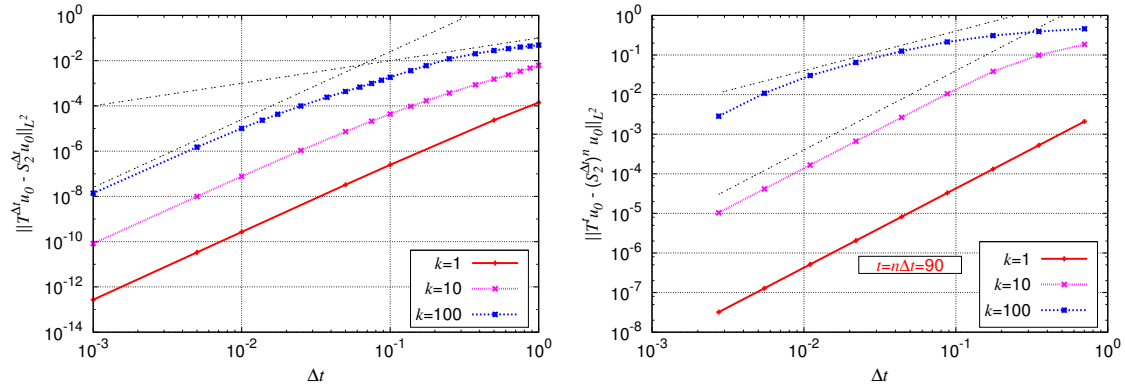
Figure 4: 1D KPP. \mathcal{S}_2 -Strang local (left) and global (right) L^2 errors for several splitting time steps \Delta t and k = 1, 10, \text{ and } 100 . Dashed lines with slopes 3 and 1 (left), and with 2 and 1 (right) are depicted.
