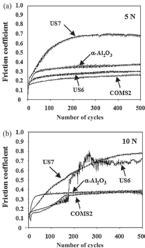
Fig. 7. Friction coefficient of the Co–Al 2 O 3 layers versus number of cycles for applied loads of 5 N (a) and 10 N (b) against an Al 2 O 3 ball.
