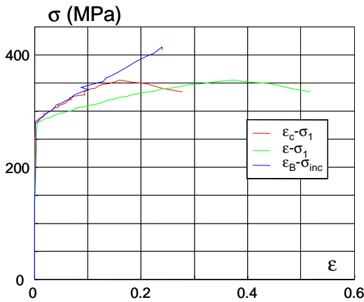
Figure 2- Mechanical response
