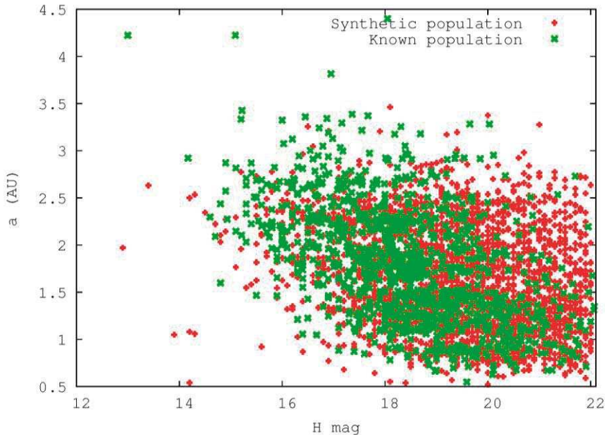
Fig. 3: Representation of the known ( \times ) and synthetic ( + ) populations possibly observed by the satellite Gaia during the mission.
