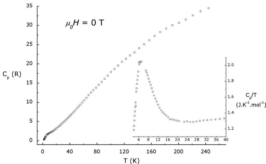
Fig. 3. \text{Pb}_{1.5}\text{Fe}_2(\text{PO}_4)_3 sintered pellet specific heat measurement.
