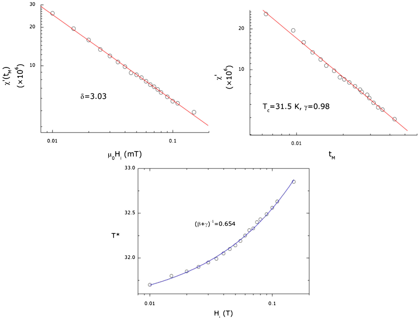
Fig. 9. The susceptibility maxima, \chi_m , as a function of internal magnetic field, H_i , and as a function of the reduced temperature, t_m , of \text{PbFe}_3\text{O}(\text{PO}_4)_3 nonoriented crystals.
