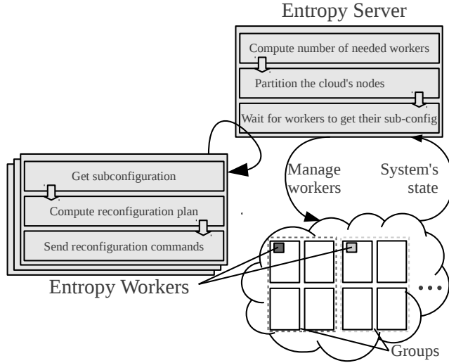
Figure 4. Dynamically Scalable Entropy
