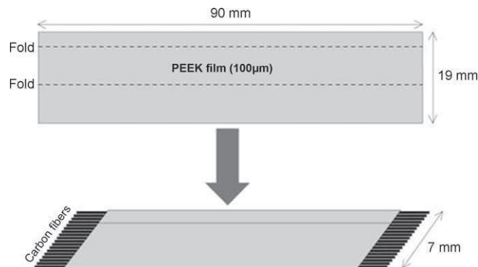
Fig. 4. Scheme of the sample preparation.
