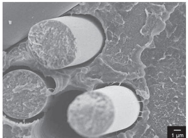
Fig. 14. Unsize carbon fiber composite.
