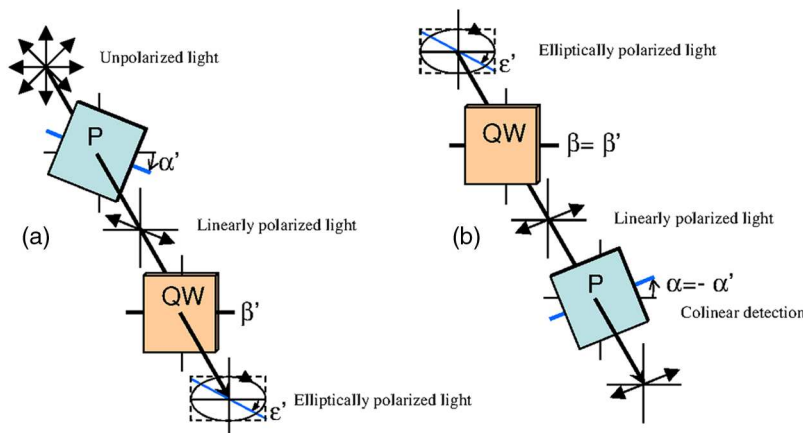
Fig. 1 Sketch of an example of the optical imaging system with linear polarizers (P) and quarter-wave plates (QW). (a) Generation of the elliptically polarized light in the illumination path. (b) Analysis of elliptically polarized light in the detection path. The polarization ellipse of the illumination and the detection can be described by the rotation angles \alpha and \alpha' of the horizontal axis of the linear polarizer and the rotation angle \beta and \beta' of the fast axis of the quarter-wave plate. The ellipticities \varepsilon and \varepsilon' are defined by \varepsilon = \beta - \alpha and \varepsilon' = \beta' - \alpha' . Copolarization detection is obtained for \alpha = \alpha' , \beta = \beta' , and \varepsilon = \varepsilon' .
