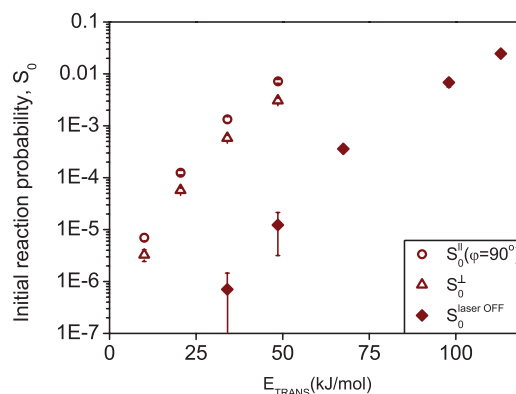
FIG. 13. Initial reaction probability of methane as a function of translational energy on Ni(110). Error bars represent \pm 95\% confidence from student-T statistics on replicate measurements.
