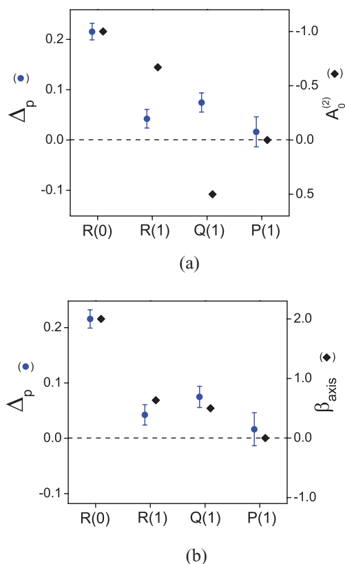
FIG. 7. Comparison of the experimentally determined \Delta_p values for \text{CH}_4(\nu_3) to (a) the corresponding calculated \vec{J} alignment coefficients A_0^{(2)} . (b) the corresponding calculated vibrational alignment coefficients \beta_{axis} . Error bars represent \pm 2\sigma of the average of 4–9 replicate measurements.
