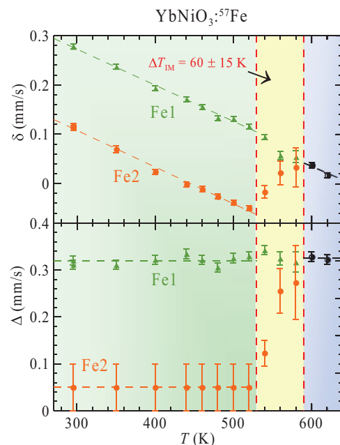
FIG. 5. (Color online) Temperature dependencies of the isomer shifts ( \delta_i ) and quadrupole splittings ( \Delta_i ) for Fe1 and Fe2 subspectra of RNi_{0.985}^{57}\text{Fe}_{0.015}\text{O}_3 ( R = \text{Tm, Yb} ).
