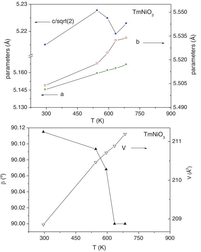
FIG. 7. (Color online) Thermal variation of the unit-cell parameters across the electronic delocalization of TmNiO 3 ( T MI = 596 K). (a) a , b , and c parameters, and (b) monoclinic \beta angle and unit-cell volume.
