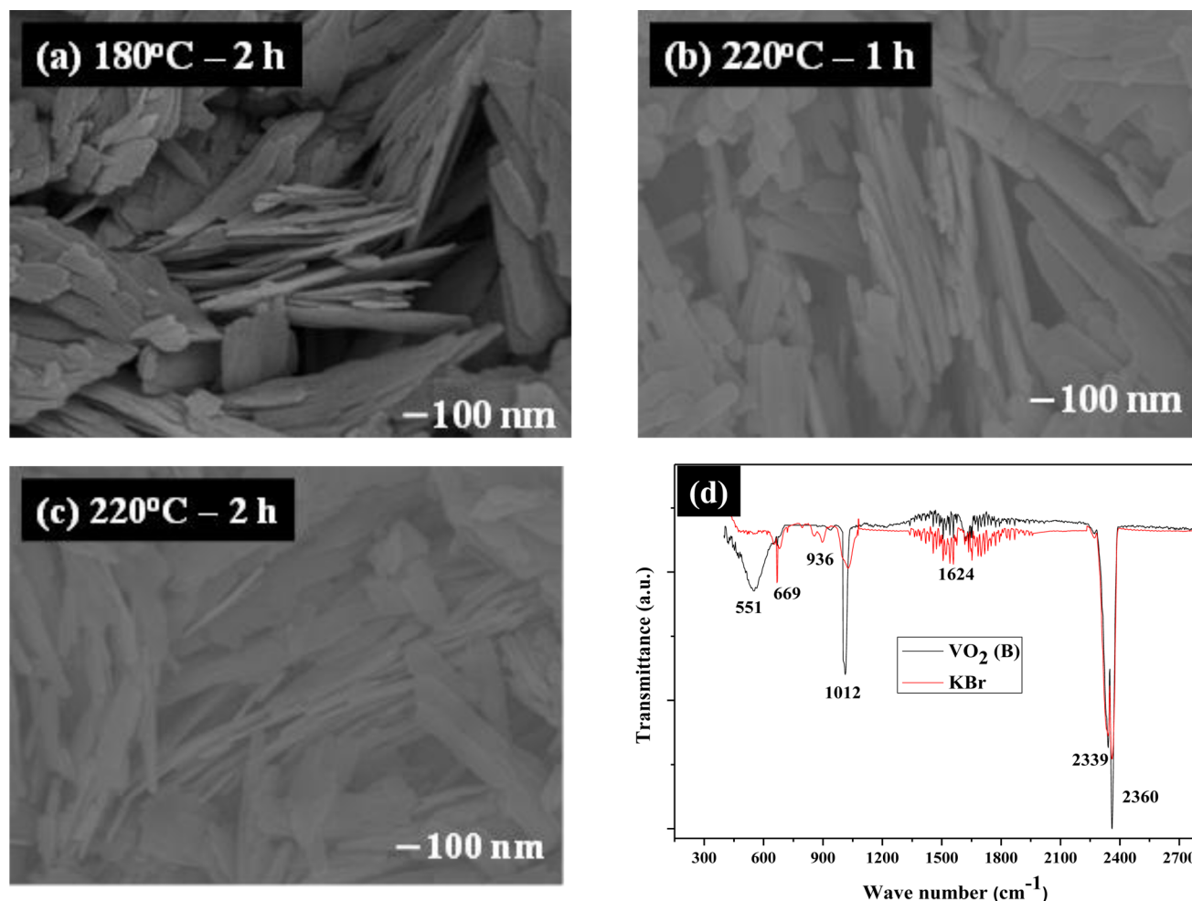
Figure 4. HRSEM images of VO 2 (B) synthesized at (a) 180 °C for 2 h, (b) 220 °C for 1 h, and (c) 220 °C for 2 h. (d) FT-IR spectra of VO 2 (B) sample prepared at 220 °C for 2 h.
