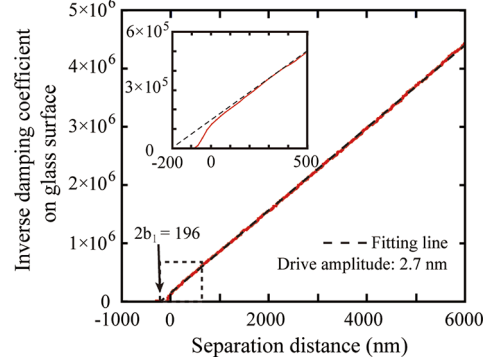
Figure 4. Inverse damping coefficient of the cantilever on a glass surface using eq 8 to fit the data and get the total slip length of 2b_1 = 196 nm. The drive amplitude of the cantilever was 2.7 nm.
