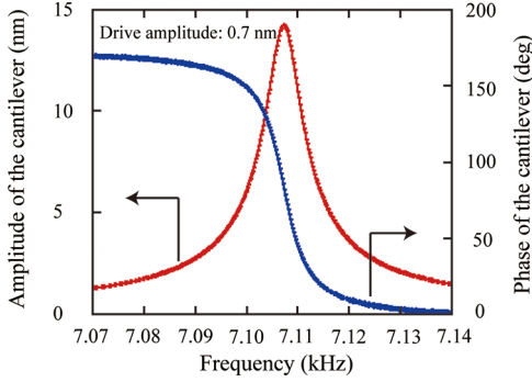
Figure 2. Amplitude and phase spectra of the cantilever with a sphere glued to the top.
