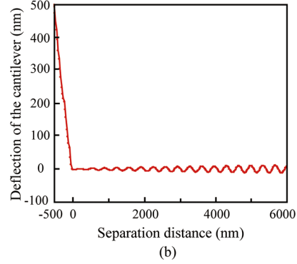
Figure 3. (a) Amplitude and phase of the cantilever measured on the mica surface. (b) Deflection of the cantilever measured as the glued sphere approaches the mica surface that allows one to determine the zero distance contact position of the two surfaces.
