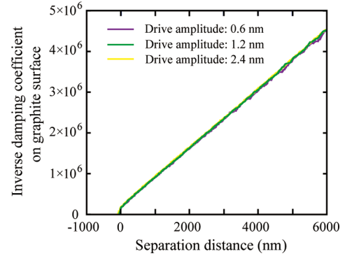
Figure 7. Inverse damping coefficient on a graphite surface with three different driving amplitudes: 0.6, 1.2, and 2.4 nm.
