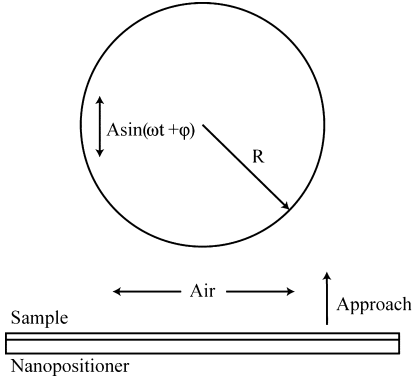
Figure 1. Schematic of a surface that is approaching an oscillating sphere with a very low velocity in air driven by a nanopositioner.
