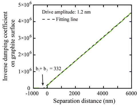
Figure 6. Inverse damping coefficient on the graphite surface using eq 9 to fit the data and get the total slip length of b_1 + b_3 = 332 nm. The drive amplitude of the cantilever was 1.2 nm.
