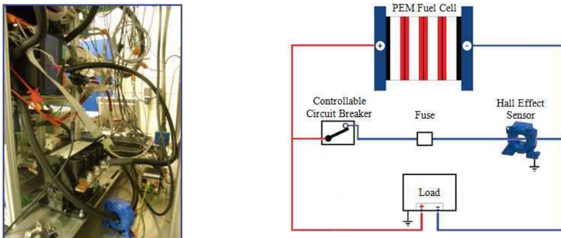
Figure 2. Short-Circuit Schema
