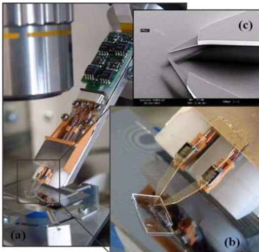
Fig. 8 a PiezoTweezer prototype, b and c details of polymer finger-tips
