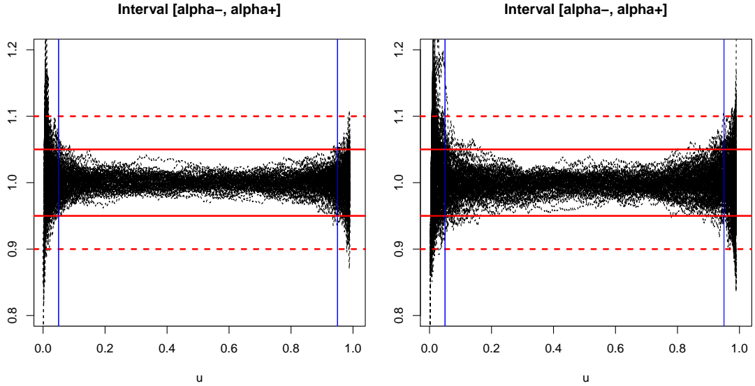
Figure 1: 100 paths of ratios a(u) = \ln \widehat{\delta}(u) / \ln \widetilde{\delta}(u) , for simulated bivariate data with Gumbel copula of parameter \theta = 2 (Kendall's \tau = 0.5 ) in the case where the data size is n = 3500 (left) or n = 2000 (right). Here we choose bounds \alpha^+ = 0.9 and \alpha^- = 1.1 (dashed horizontal lines) and \alpha^+ = 0.95 and \alpha^- = 1.05 (full horizontal lines). The blue vertical lines represents the considered interval I = [0.05, 0.95] \subset [0, 1] .
