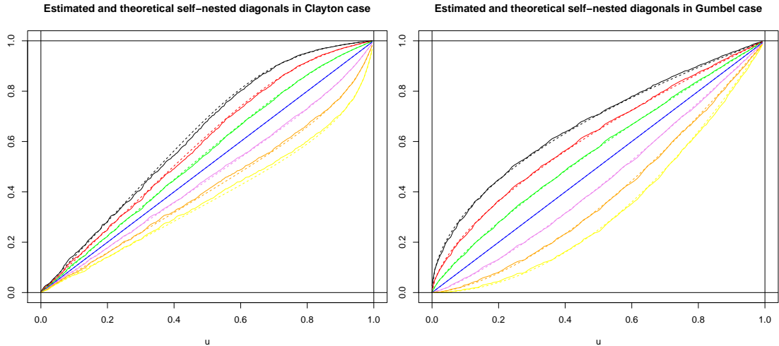
Figure 2: Estimation of self-nested diagonal \widehat{\delta}_k(u) as in Definition 4.1 in the Clayton-case with parameter \theta = 6 (left), or in the Gumbel-case with parameter \theta = 3 (right) for k = -3, -2, -1, 0, 1, 2, 3 . The estimated \widehat{\delta}_k(u) are represented using full lines, the theoretical one's using dotted lines. The black upper curve corresponds to k = -3 , the yellow lower curve to k = 3 .
