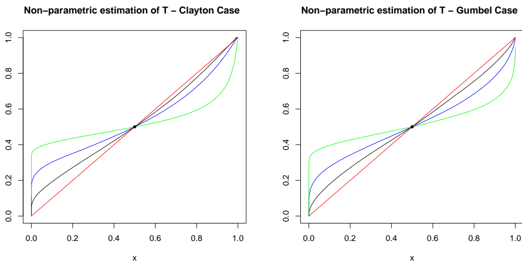
Figure 3: Non-parametric \hat{T}(x) as in Definition 4.2 estimated on a sample of size n = 1500 . Bivariate Clayton-case (left) and bivariate Gumbel-case (right) with Kendall's \tau = 0.25 (black lines), \tau = 0.5 (blue lines), \tau = 0.75 (green lines). The red line represents the bisectrix of the quadrant. Each transformation T(x) is passing through the point (0.5, 0.5) (black point).
