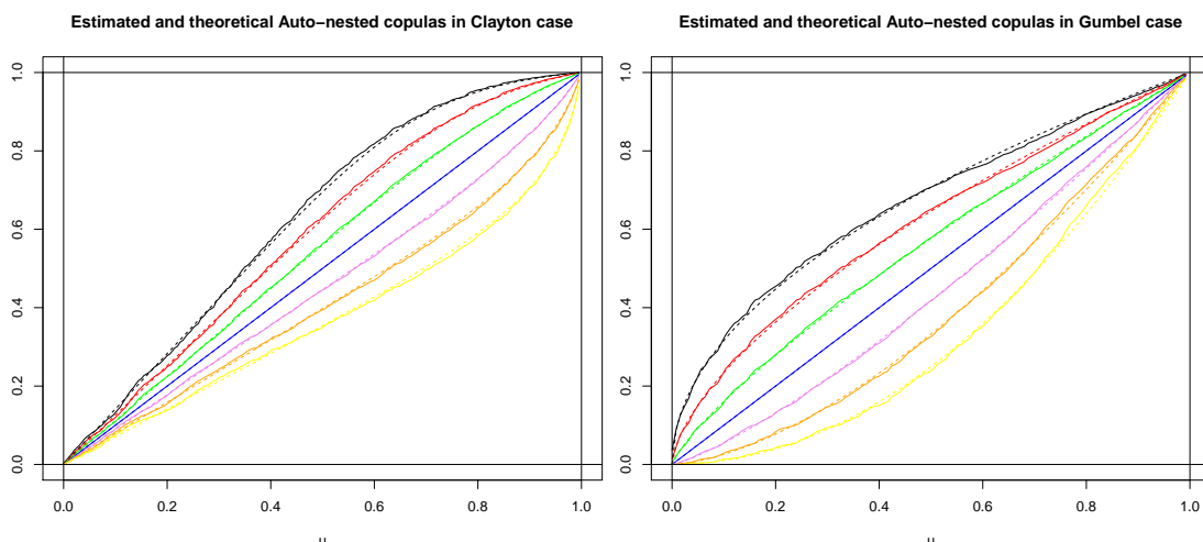
Figure 2: Estimation of self-nested copula \hat{\delta}_k(u) as in Definition 4.1 in the Clayton-case with parameter \theta = 6 (left), or in the Gumbel-case with parameter \theta = 3 (right) for k = -3, -2, -1, 0, 1, 2, 3 . The estimated \hat{\delta}_k(u) are represented using full lines, the theoretical one's using dotted lines. The black upper curve corresponds to k = -3 , the yellow lower curve to k = 3 .
