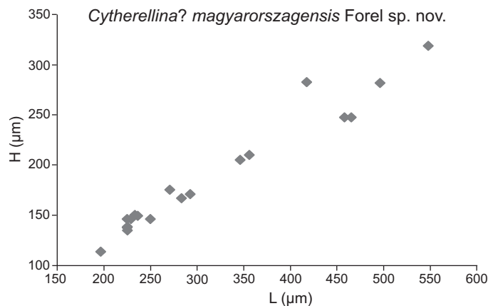
Fig. 14. Height/length diagram of Cytherellina? magyarorszagensis Forel sp. nov.
