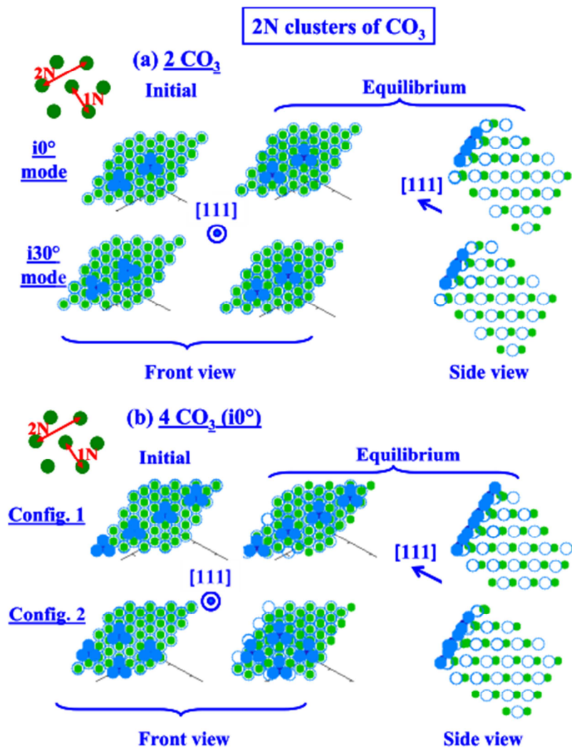
Figure 8 : Insertion of 2N clusters of \text{CO}_3 within the (111) surface of CaO (L0 layer): initial configurations (left) and relaxed ones (middle and right).
