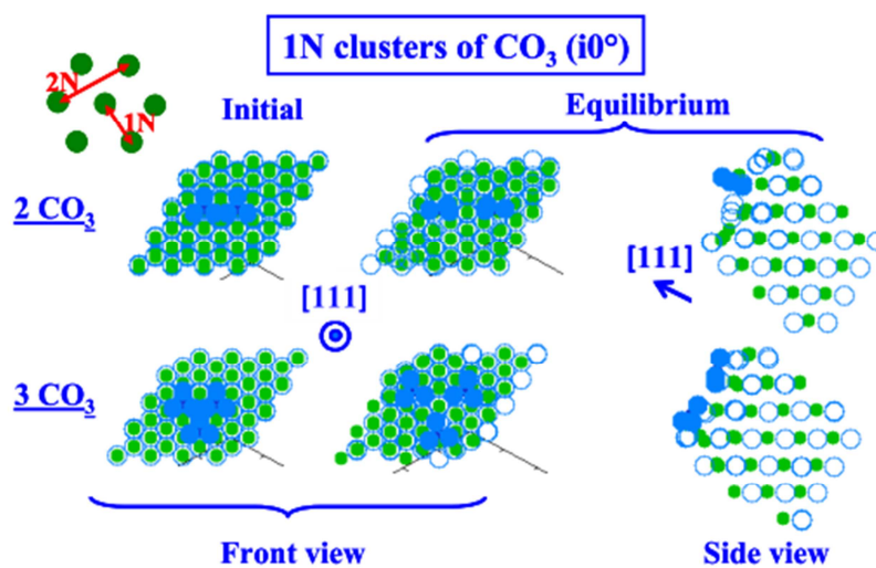
Figure 7 : Insertion of 1N clusters of CO 3 within the (111) surface of CaO (L0 layer): initial configurations (left) and relaxed ones (middle and right).
