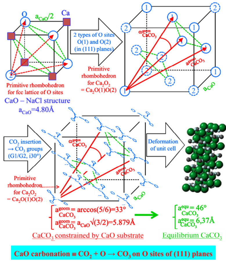
Figure 1 : Schematics of the carbonation process of calcium oxide, with CO_2 + O \rightarrow CO_3 substitutions leading to calcite.
