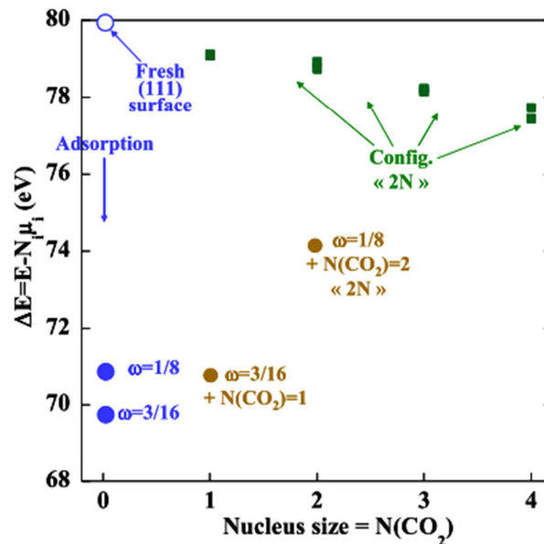
Figure 9 : Adsorption-insertion energetics for CO 2 in the (111) surface of CaO ; \omega refers to various levels of adsorption.
