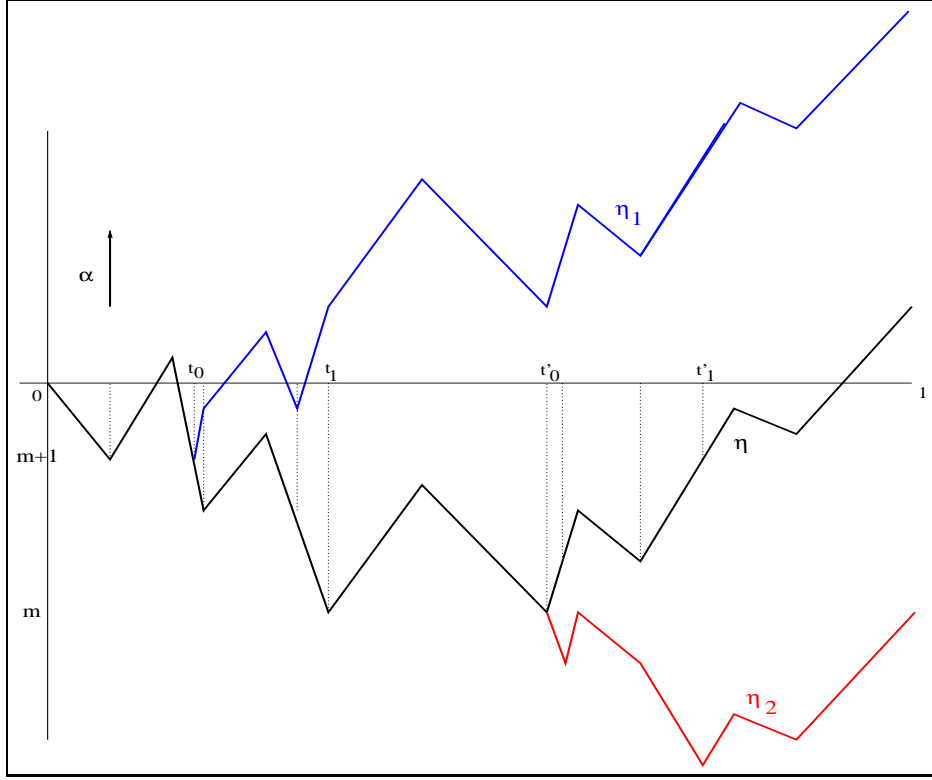
FIGURE 1. Paths \eta , \eta_1 = \tilde{e}_i(\eta) and \eta_2 = \tilde{f}_i(\eta)
