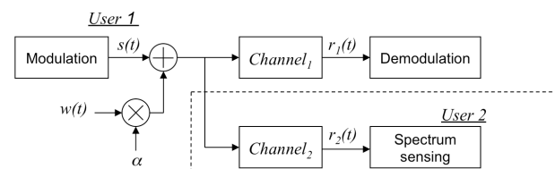
Fig. 1. System model of the watermark insertion in the signal of User 1 and its detection by User 2.
