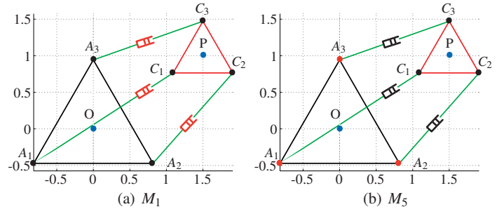
Figure 8. Two actuating modes: (a) 3- \underline{R} PR manipulator, (b) 3- \underline{R}\underline{P} R manipulator, \phi = 0 and \mathbf{p} = [1.5, 1]^T
