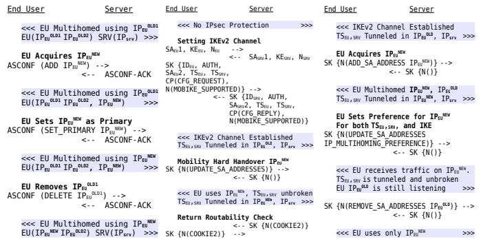
(a) SCTP Soft Hand-Over (b) MOBIKE(-X) Hard Hand-Over (c) MOBIKE-X Soft Hand-Over
