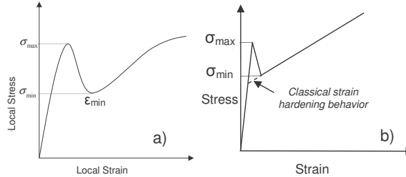
Figure 2: Two local behavior laws used to simulate Lüders' bands. Introducing local softening allows strain to localize.
