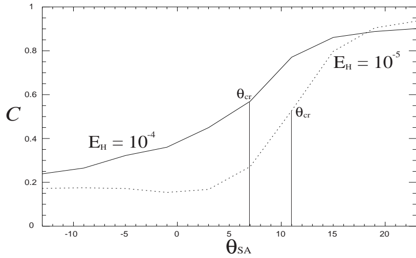
Fig. 7. The Circumglobal Flow Index ( C ) for various extensions of Eurasia towards the south, represented by \theta_{SA} . The solid curve is computed for E_H = 10^{-4} and the dashed curve for E_H = 10^{-5} .
